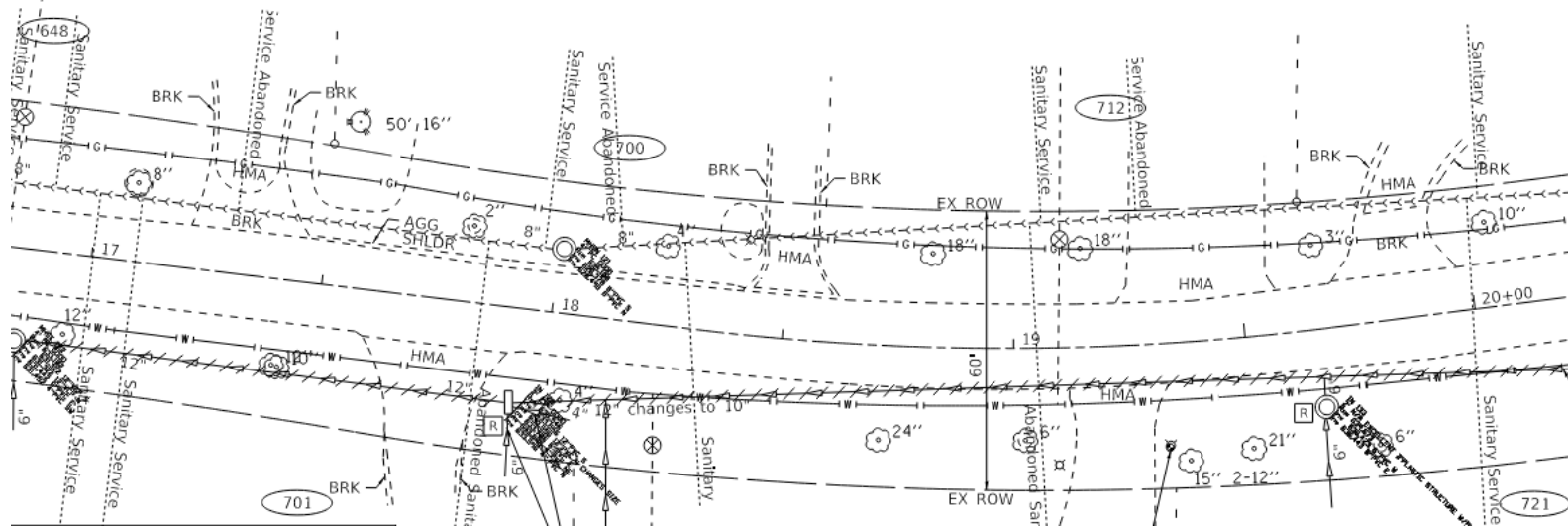
EXISTING PLAN CHATHAM ROAD
