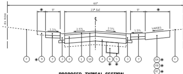
PROPOSED TYPICAL SECTION WASHINGTON STREET
