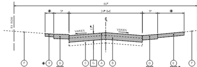
EXISTING TYPICAL SECTION WASHINGTON STREET
