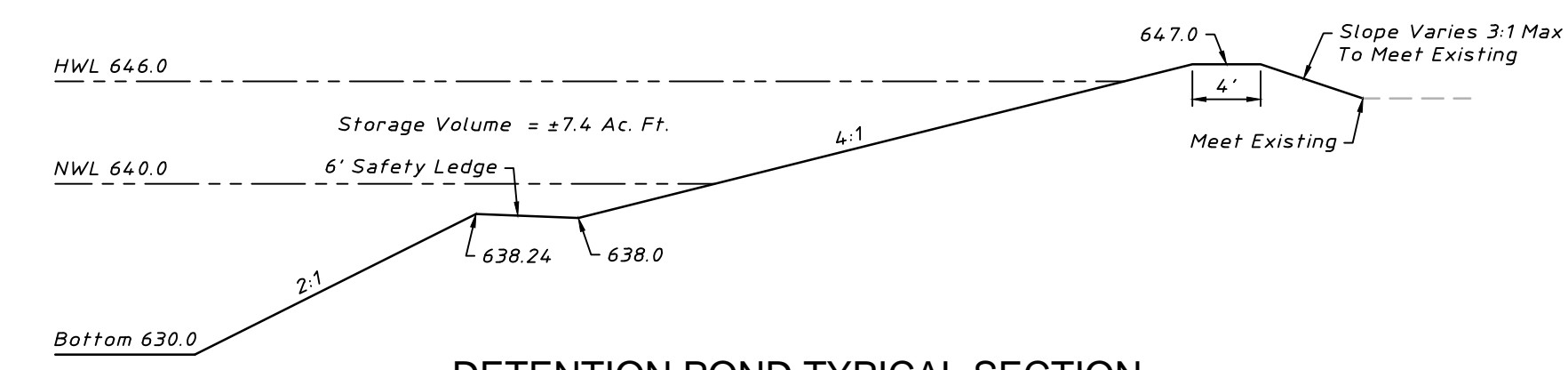
DETENTION POND TYPICAL SECTION
